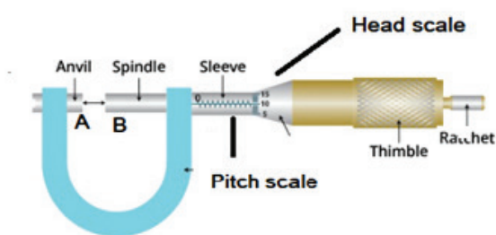
Figure 1.1 Screw gauge and its parts
