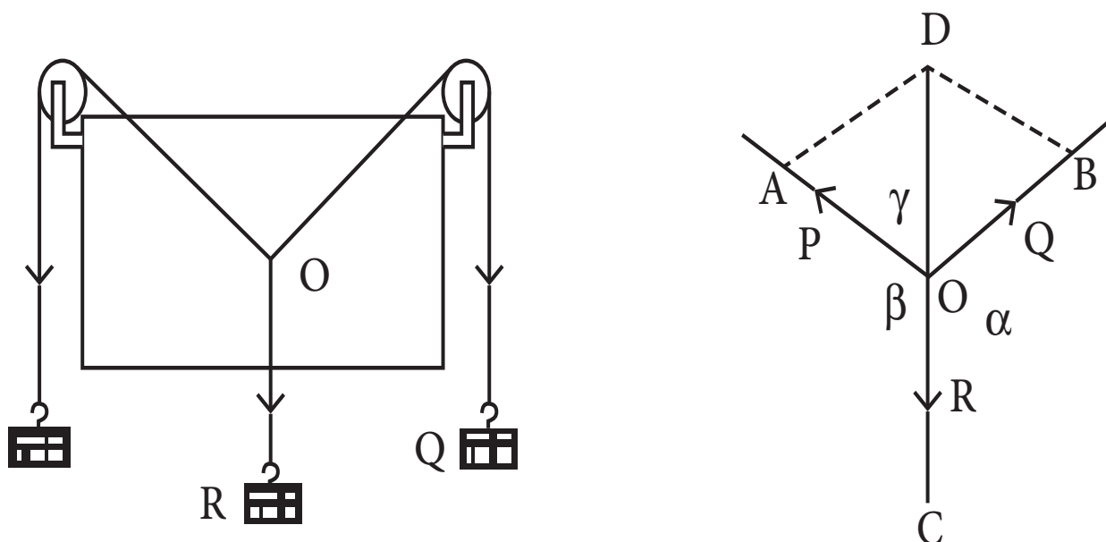
Figure 2.9 Experimental set up for verification of parallelogram law
