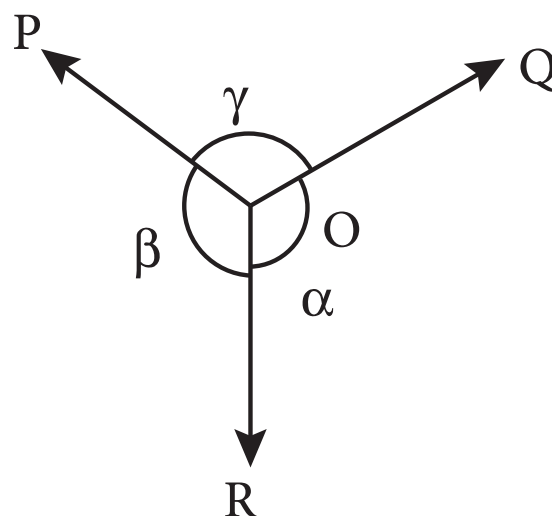
Figure 2.8 Lami's theorem
