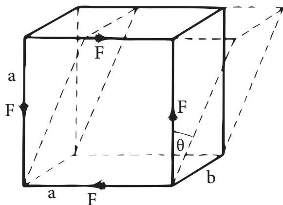
Figure 4.6 Shear strain
